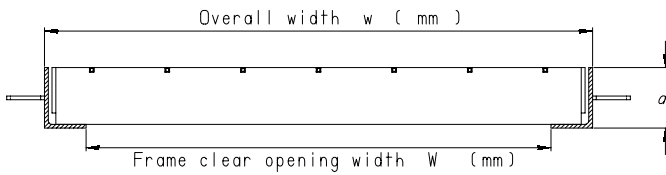
STANDARD section A-A
